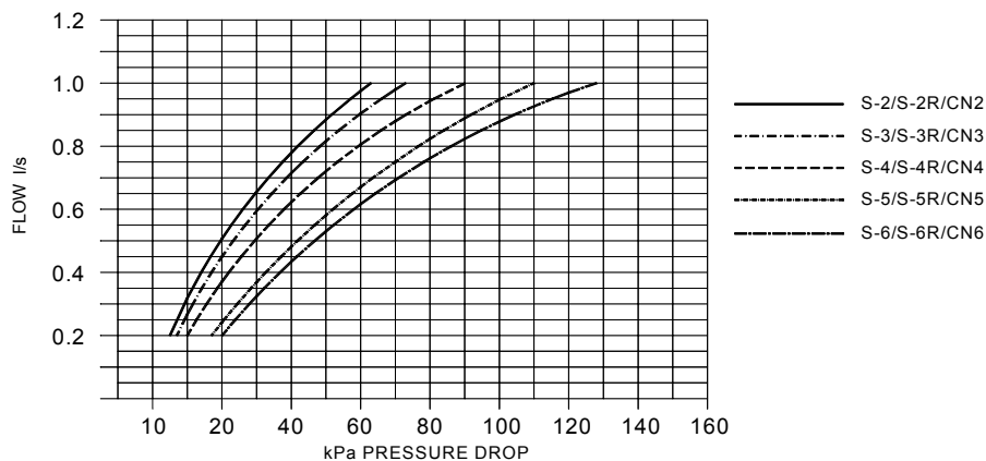
SINGLE HEAT EXCHANGER MODELS (PARALLEL FLOW)
