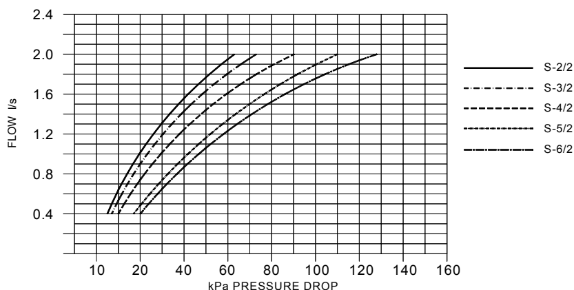
DOUBLE HEAT EXCHANGER MODELS (PARALLEL FLOW)
