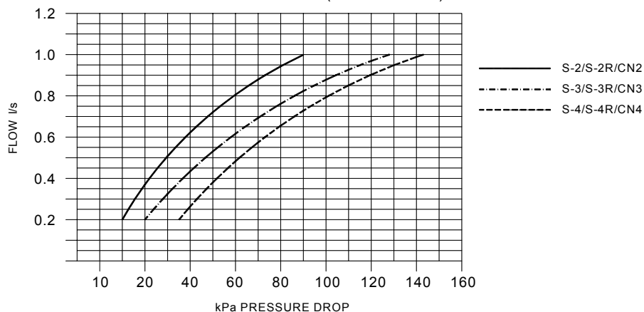
SINGLE HEAT EXCHANGER MODELS (SERIES FLOW)
